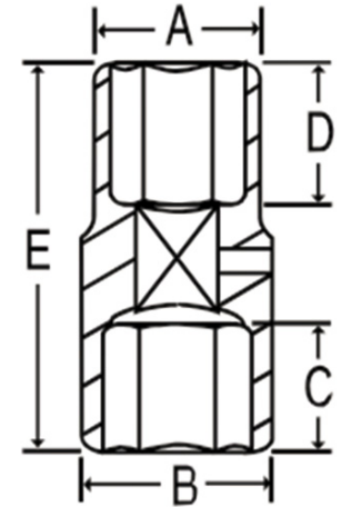
Dimensions (Inches)
